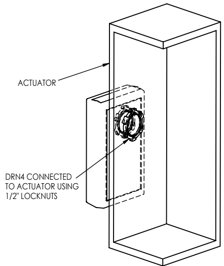
FIGURE 2: MOUNTING
