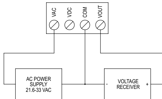
Figure 3: AC wiring
