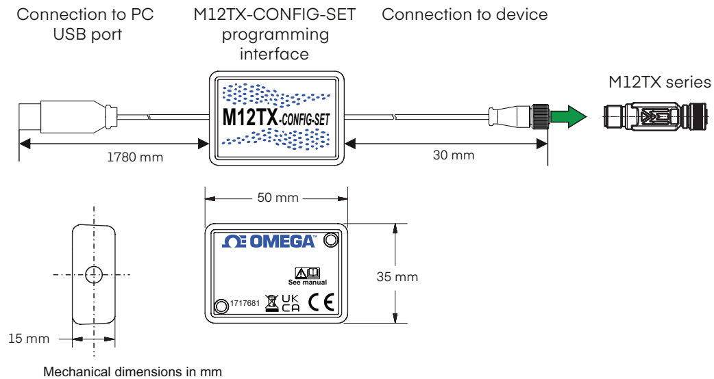
Figure 1: M12TX-CONFIG-SET mechanical dimensions
