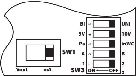
FIGURE 6: SW1 and SW3 OUTPUT SWITCHES
