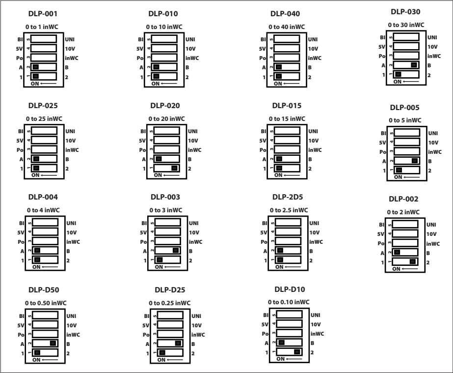
FIGURE 9: SWITCH SETTINGS
