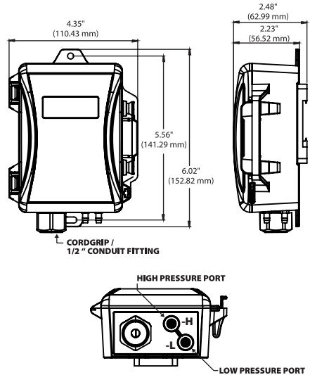
FIGURE 1: DLP DIMENSIONS
