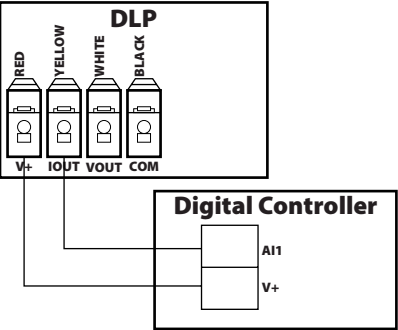
FIGURE 7: WIRING CONNECTIONS
