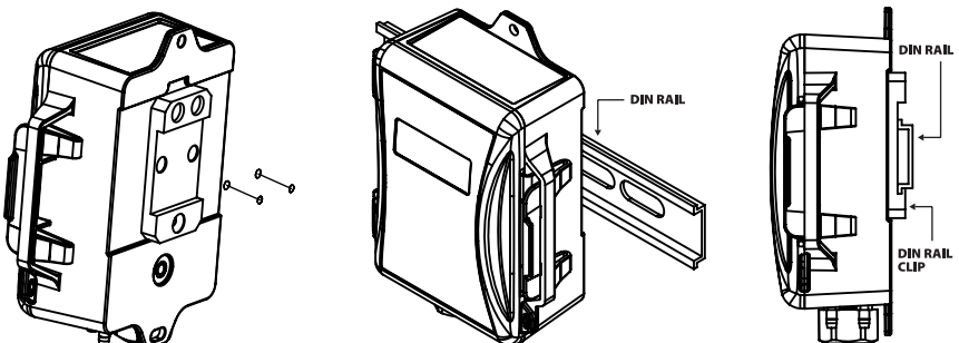
FIGURE 2: DIN RAIL MOUNTING
