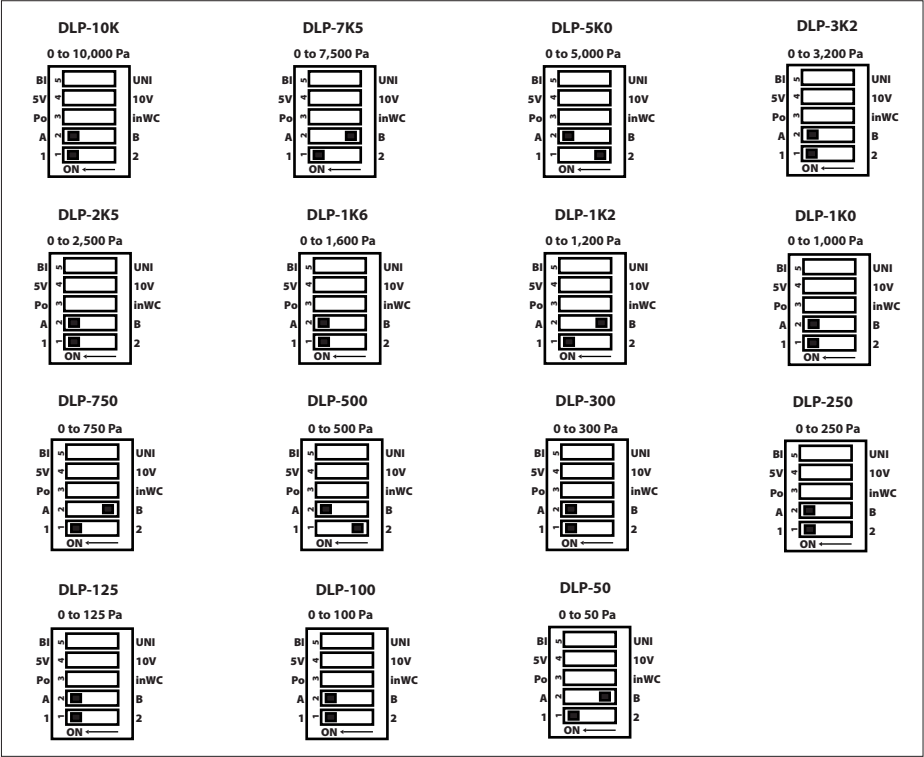
FIGURE 10: PASCALS SWITCH SETTINGS
