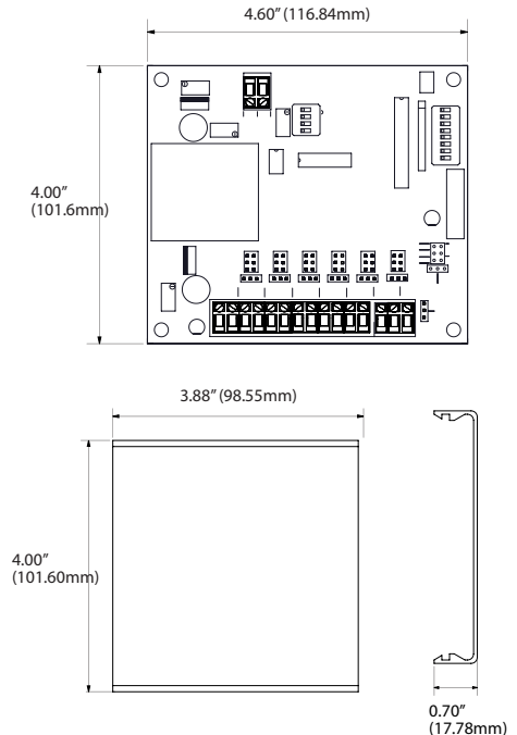
FIGURE 1: DIMENSIONS
