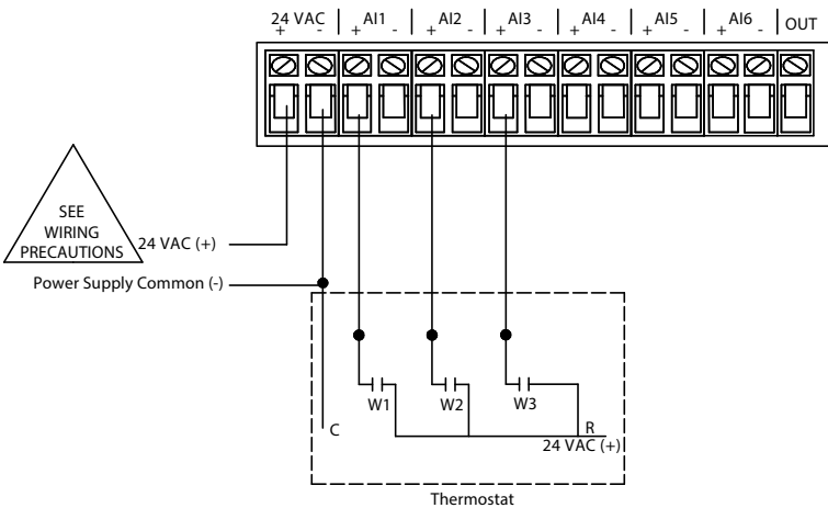
FIGURE 3: TYPICAL DIGITAL INPUTS
