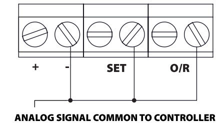
FIGURE 5: COMMON OUTPUT TO CONTROLLER
