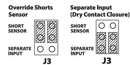
FIGURE 4: OVERRIDE OPTIONS JUMPER SETTINGS (J3)
