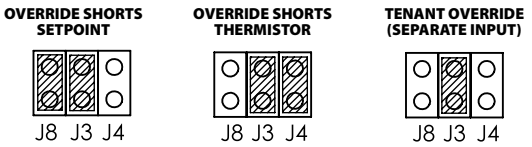
FIGURE 4: OVERRIDE OPTIONS JUMPER SETTINGS
