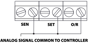
FIGURE 5: COMMON OUTPUT TO CONTROLLER
