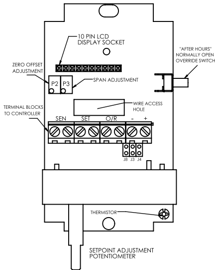
FIGURE 3: LAYOUT
