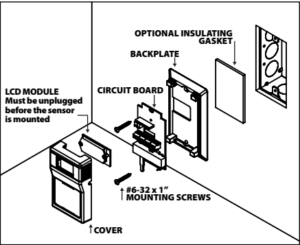
FIGURE 2: MOUNTING
