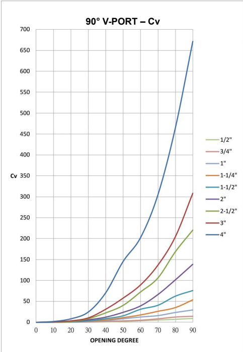
Cv Valve Charts
