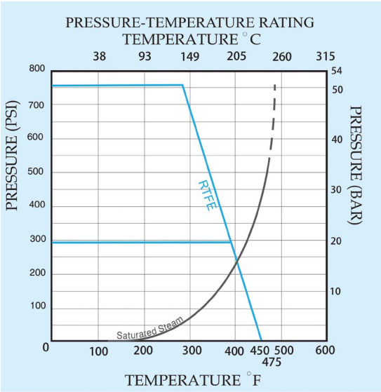
Pressure/Temperature Rating Chart
