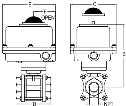
WITH EXPLOSION-PROOF ELECTRIC ACTUATOR
