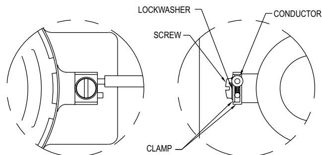
Front view detail
