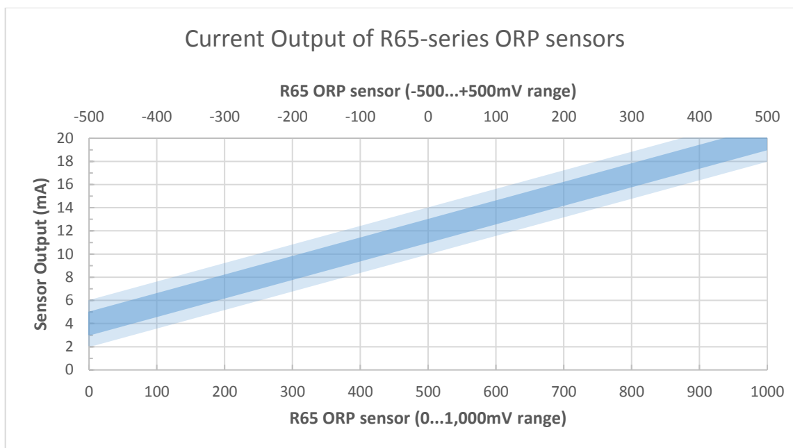
Figure 4 - Range of acceptable output for new R65 (ORP) probes. The dark blue middle band is for new probes and represents the acceptance criterion for new probes. The light blue outer band shows the acceptance criteria for working probes.
