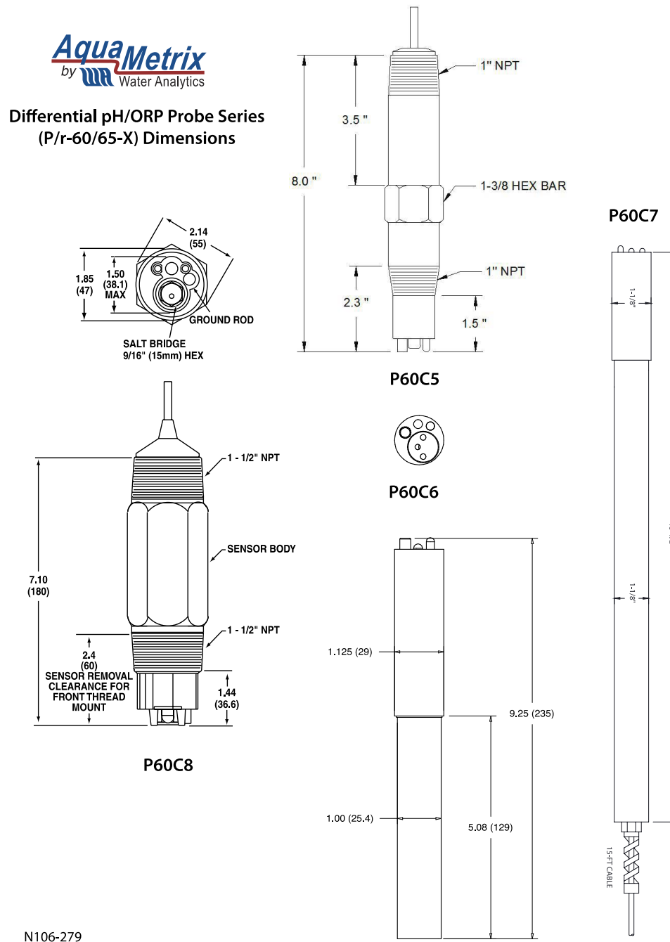
Figure 8-1 - Dimensions of -5, -6, -7 and -8 probes.
