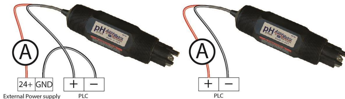
P65-Sensor with Current Sinking PLC
