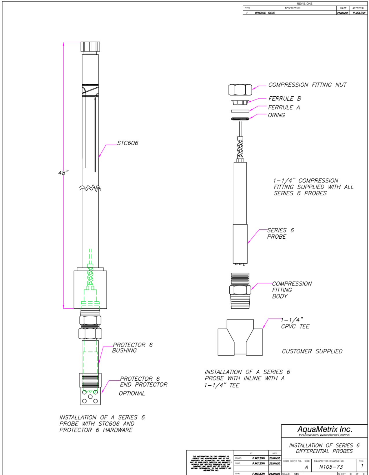
Figure 8-2 - Installation of a series 6 differential probe.
