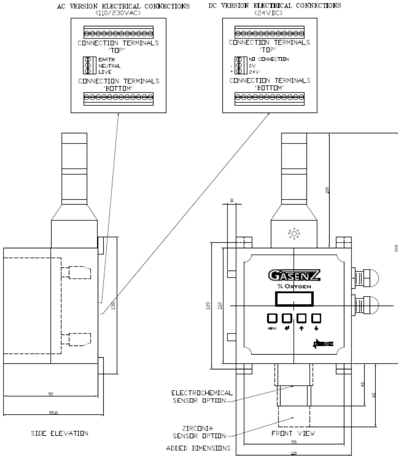
GASENZ ANALYSER GENERAL ARRANGEMENT
