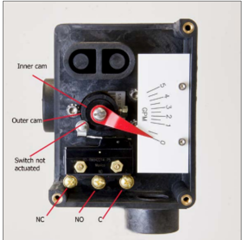
Figure 2: Device overview
