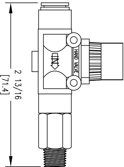
MODELS WITH EXTENSION
