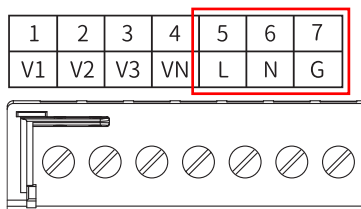
Fig. 2-7 Power Supply Wiring
