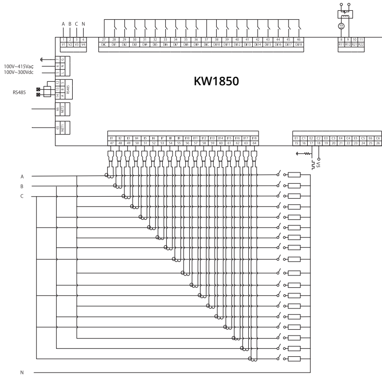
Fig. 2-9 3-Phase 4-Wire
