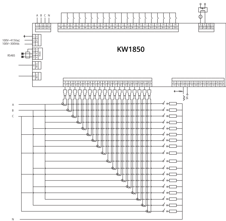
Fig. 2-8 Single Phase
