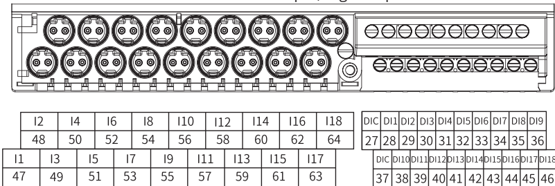
Fig. 2-6 KW1850 Terminals
