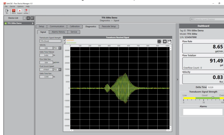
Figure 2: SoloCUE diagnostics screen
